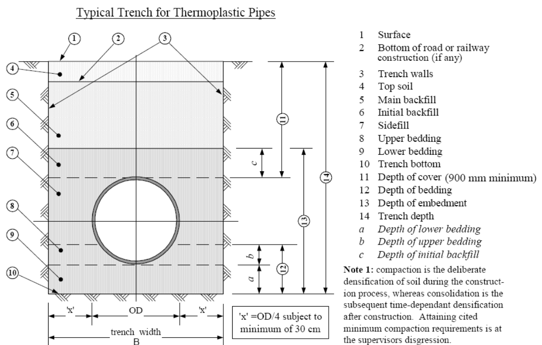
Figure: Trench Installation
